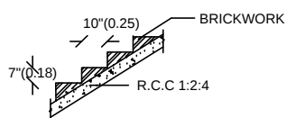
STAIRCASE WAIST SLAB
