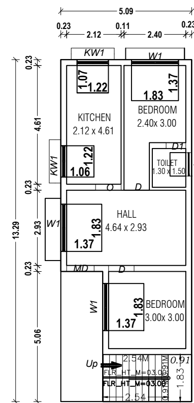
PRO. GROUND FLOOR PLAN
