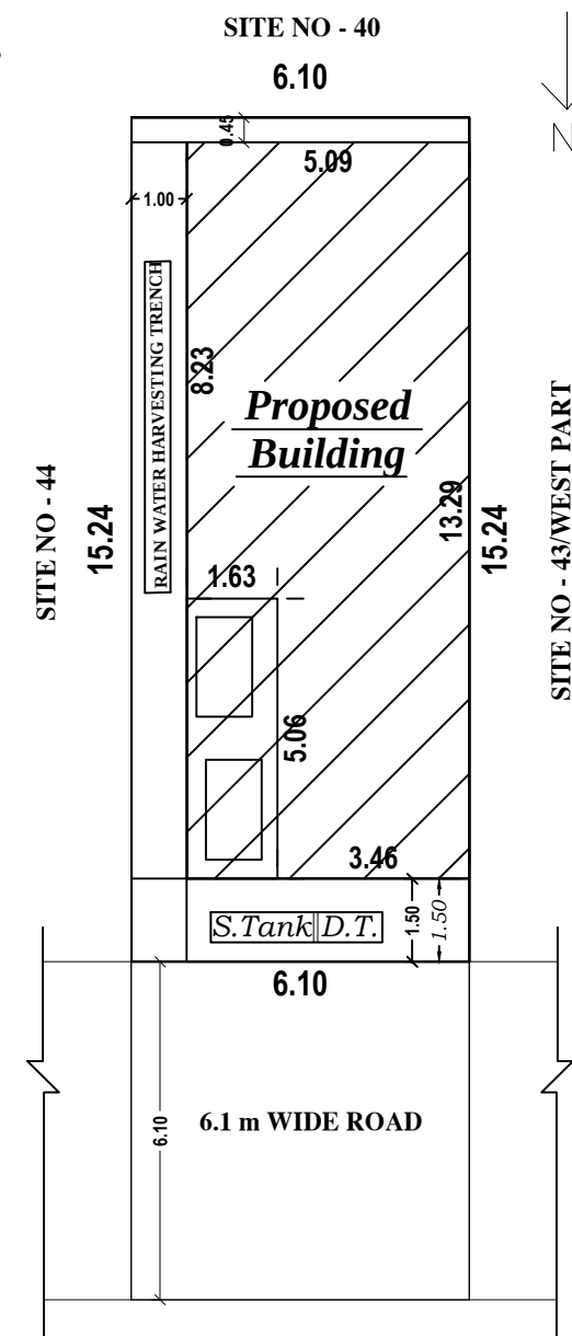
SITE PLAN
