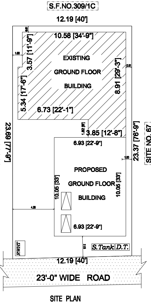
SITE PLAN
