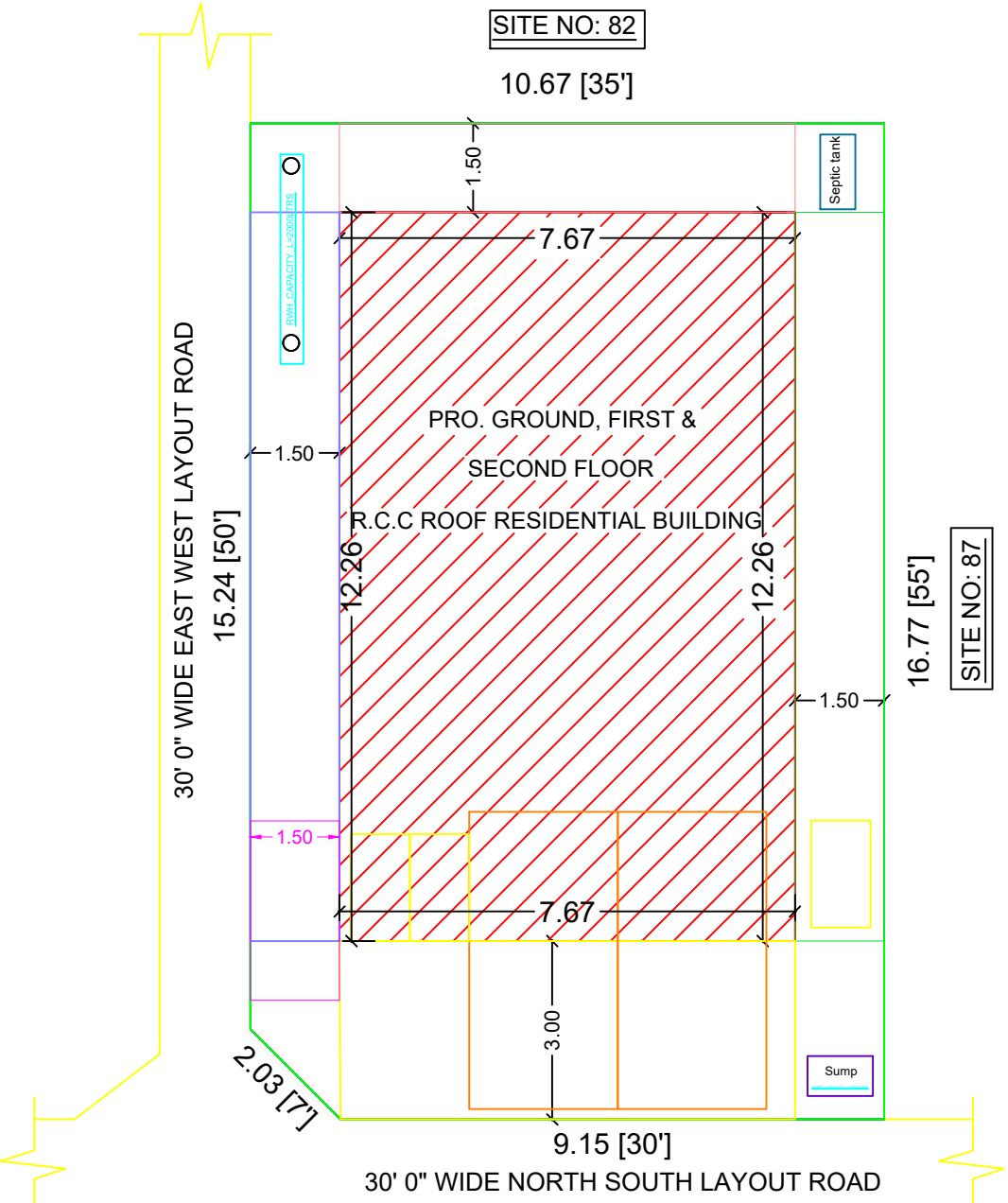
SITE PLAN
