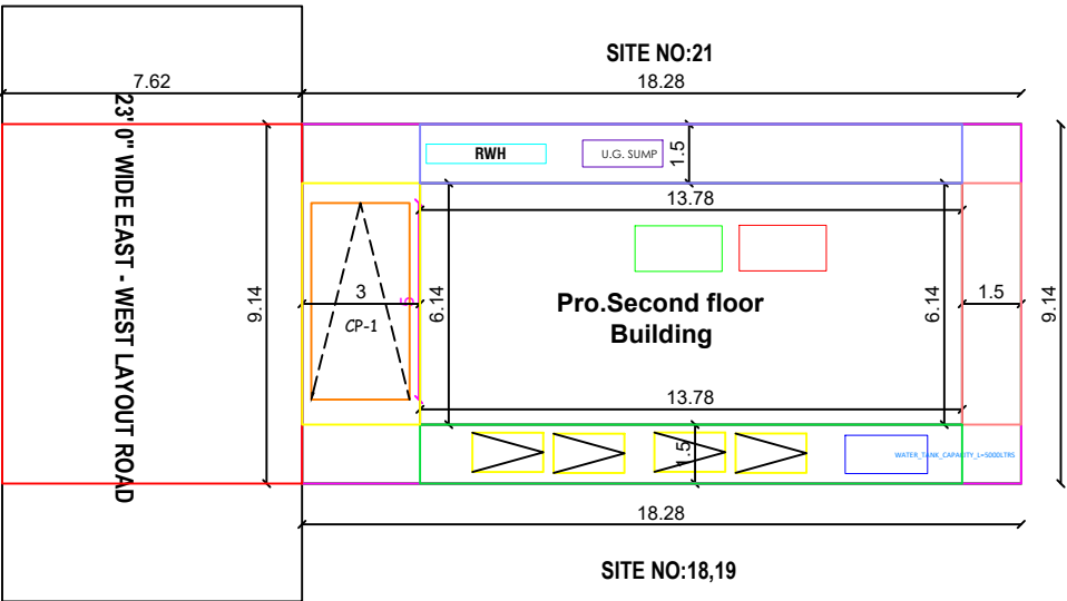
SITE PLAN (SCALE 1" : 8' 0")
