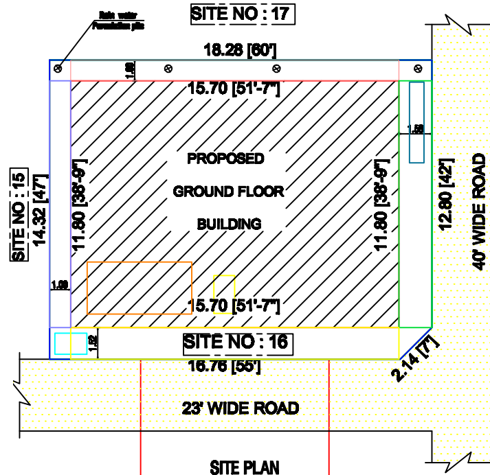
SITE PLAN
