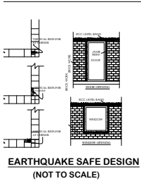
SEISMIC REINFORCEMENT DETAILS (NOT TO SCALE)
