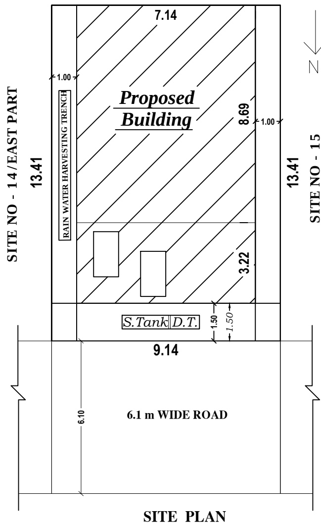
SITE PLAN
