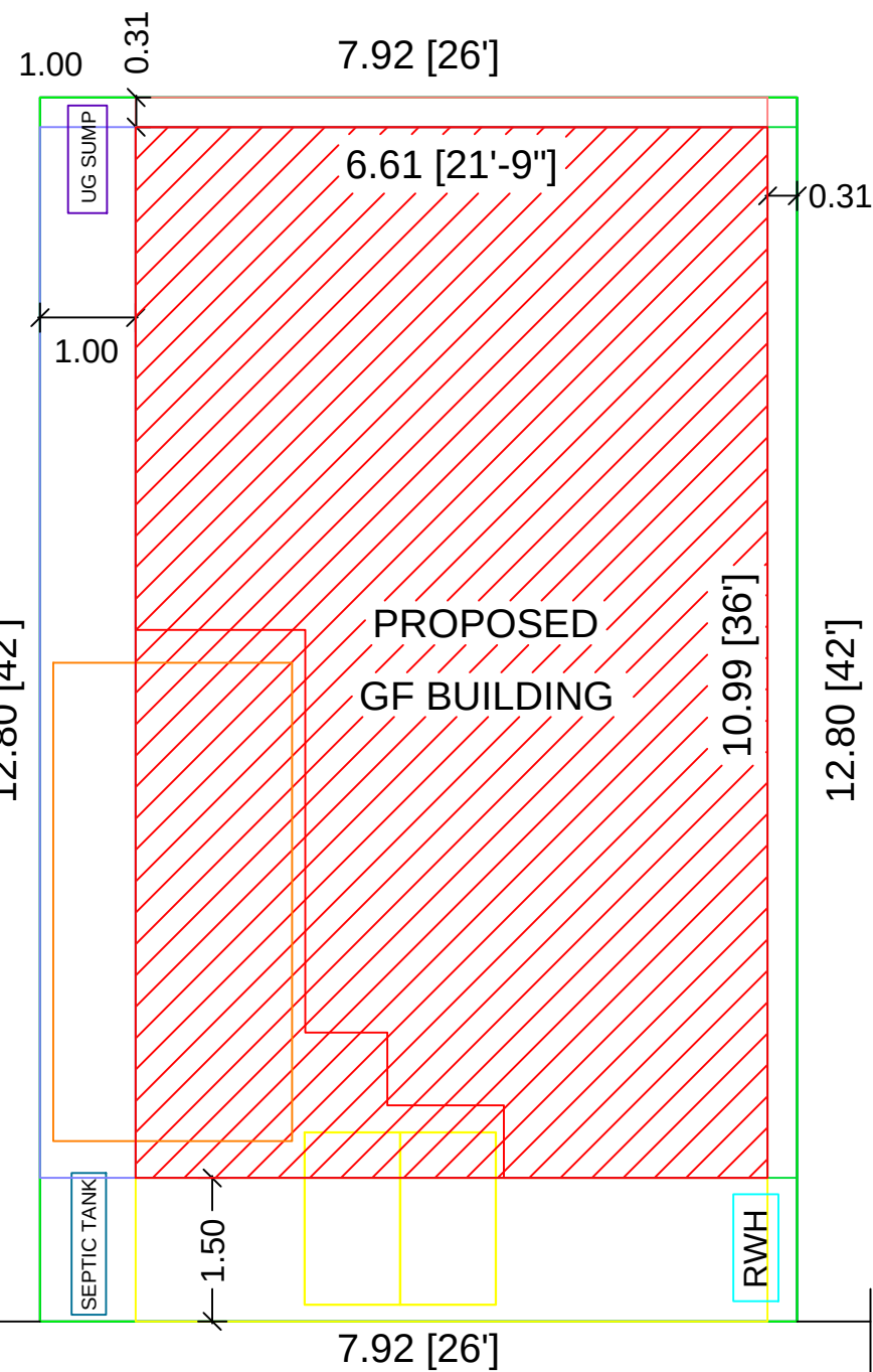
SITE PLAN
