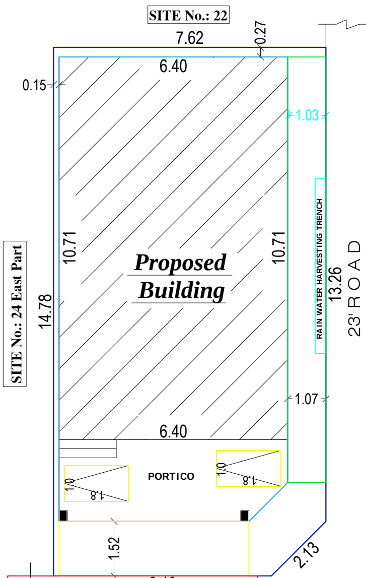
SITE PLAN
