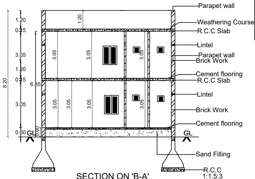
SECTION ON 'B-A'
