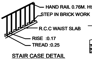
STAIR CASE DETAIL
