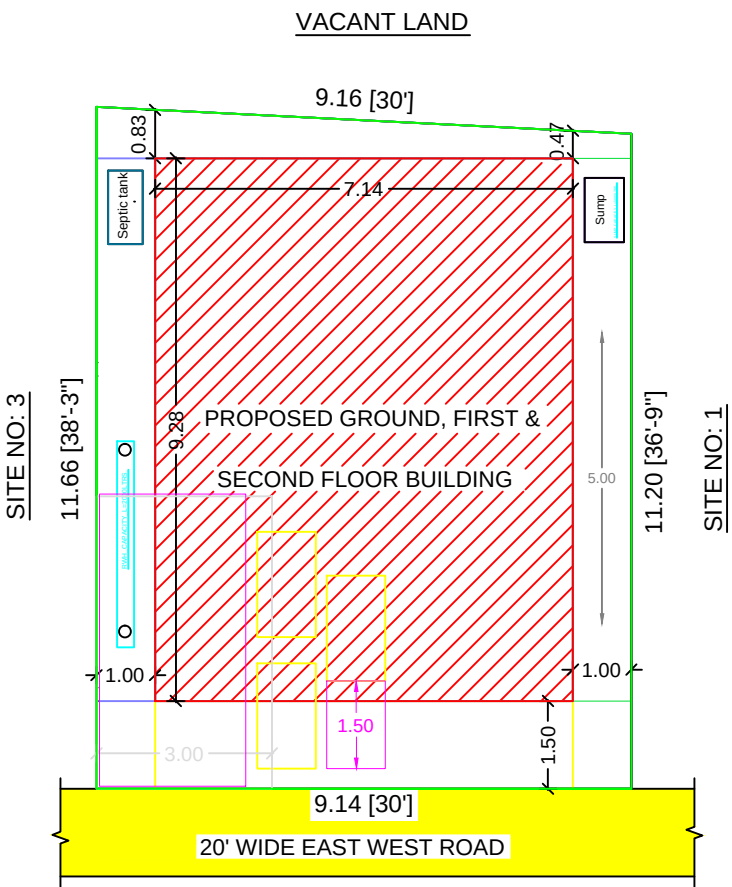
SITE PLAN
