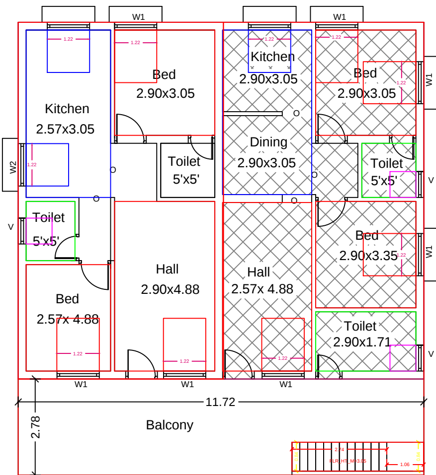
EXI. & PRO. FIRST FLOOR PLAN
