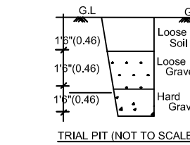
TRIAL PIT (NOT TO SCALE)
