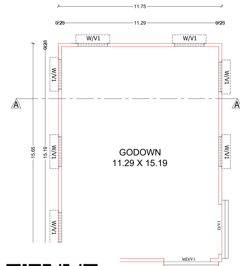
ND FLOOR PLAN
