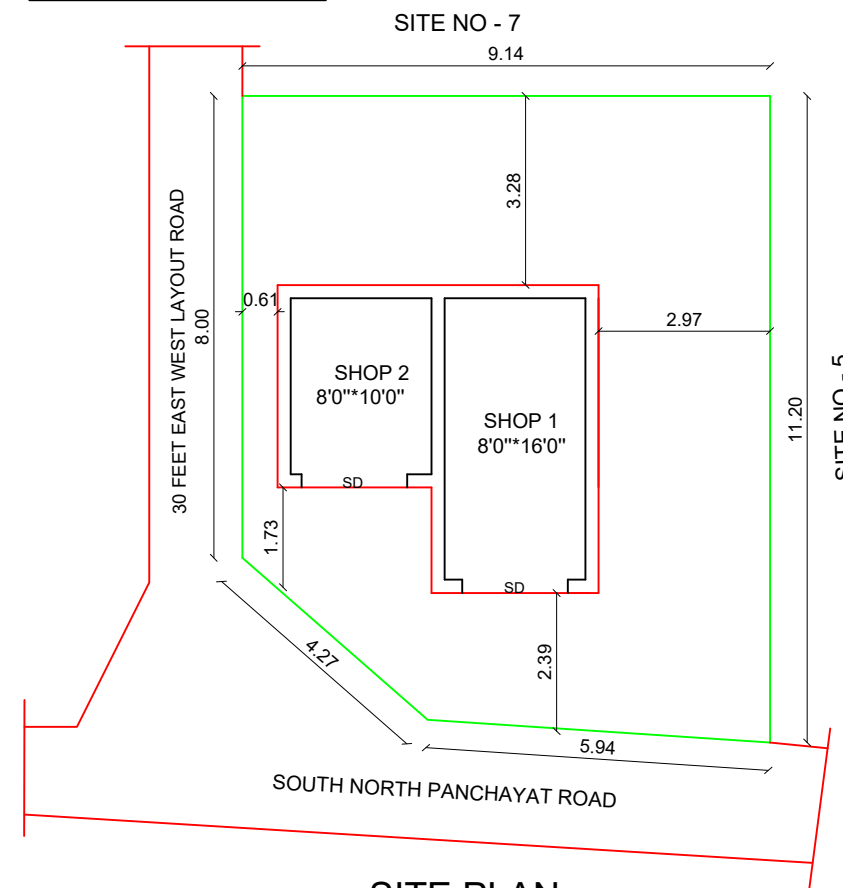
SITE PLAN
