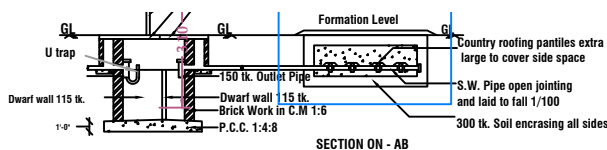
SEPTIC
