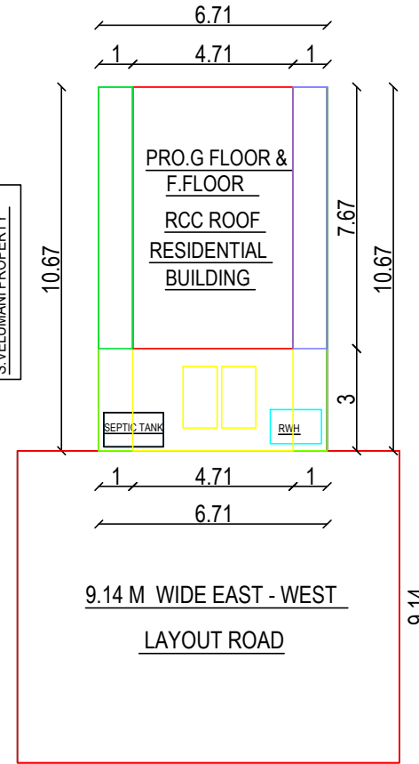
SITE PLAN
