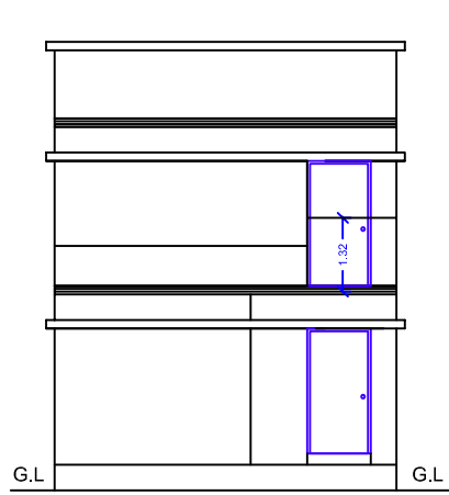
FRONT ELEVATION - A
