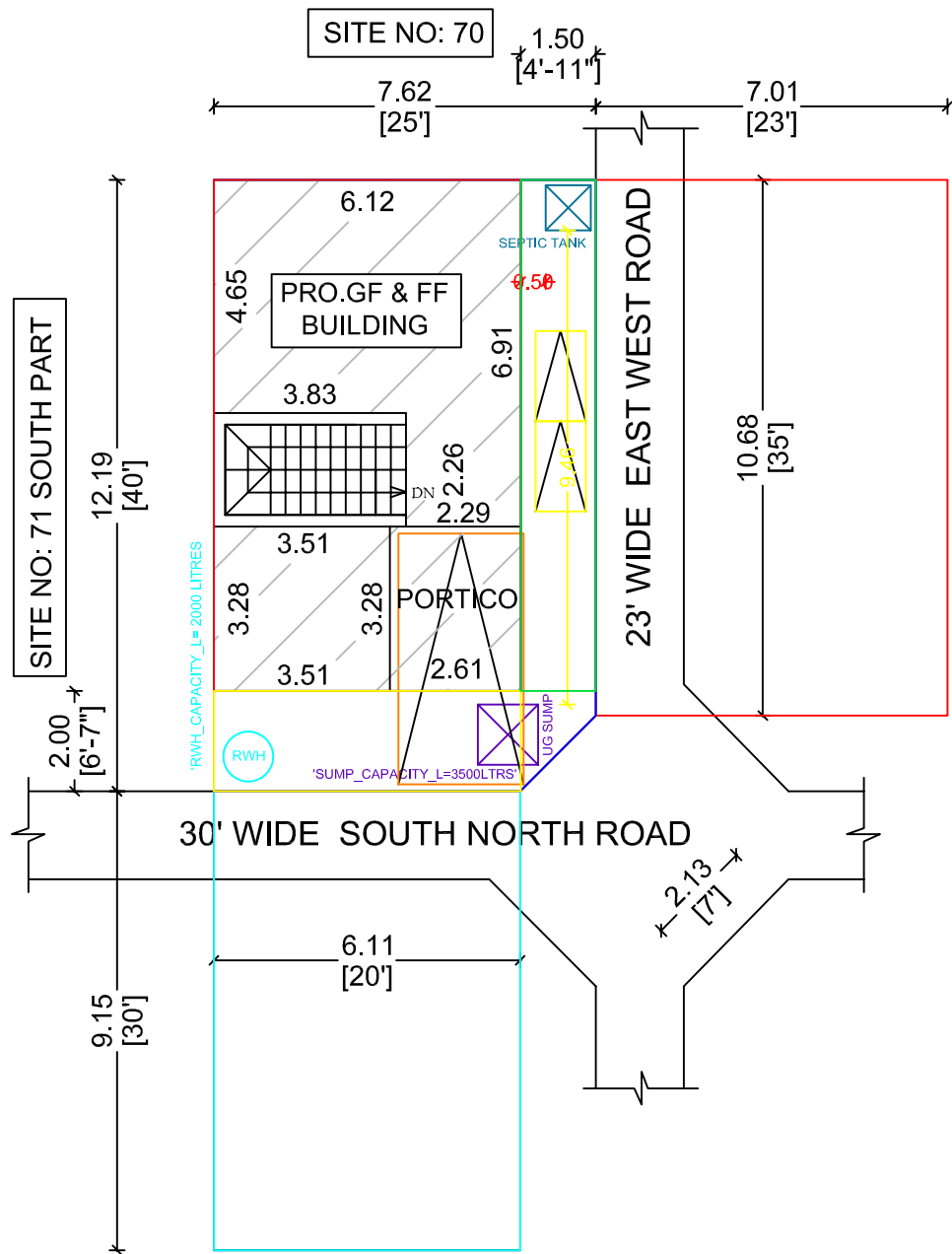
SITE PLAN
