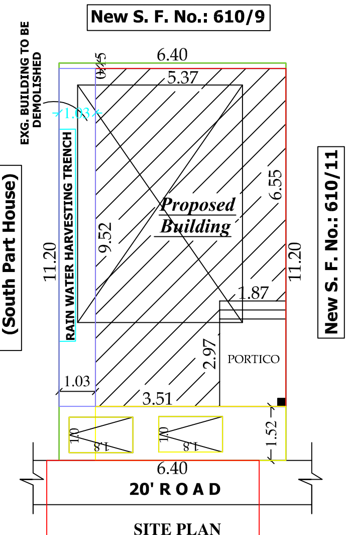
SITE PLAN
