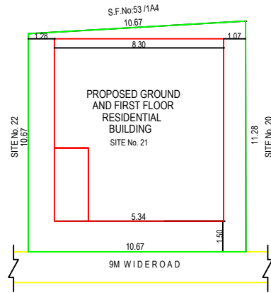
SITE PLAN
