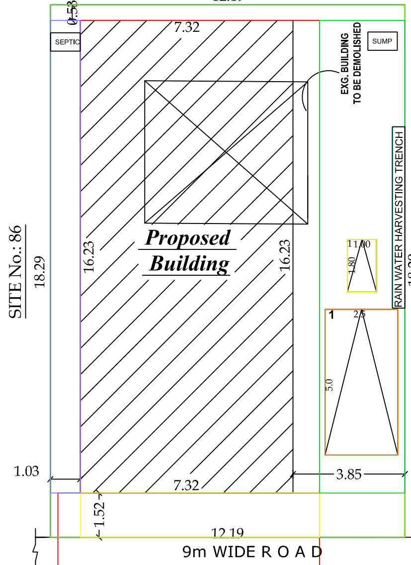
SITE PLAN
