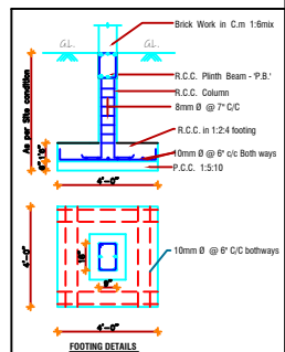
FOOTINGS DETAILS
