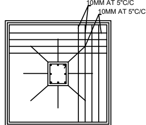
FOOTING DETAIL SCALE:
