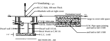
SEPTIC TANK WITH DISPEL
