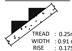
STAIRCASE DETAIL:
