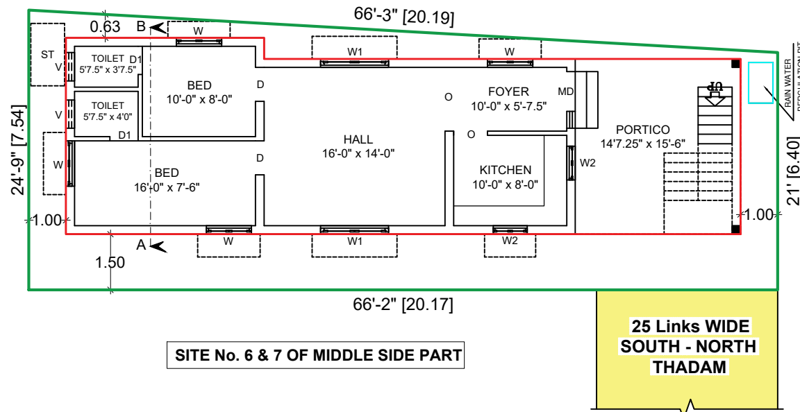
SITE CUM GROUND FLOOR PLAN
