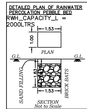
DETAILED PLAN OF RAINWATER PERCOLATION PEBBLE BED
