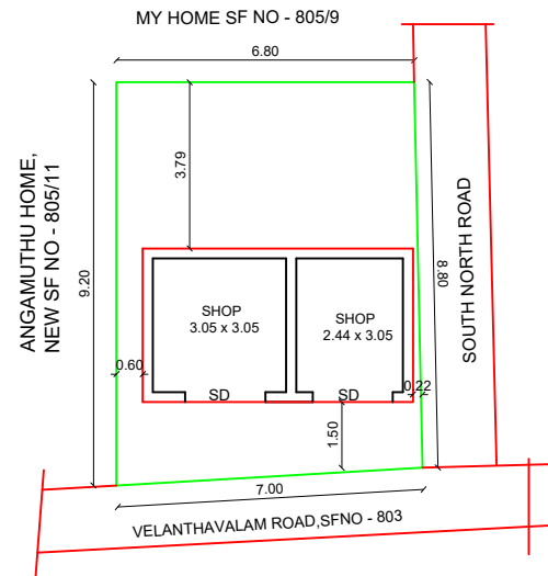
SITE PLAN
