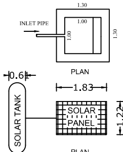
SOLAR SYSTEM
