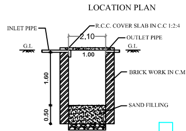
RAIN WATER COLLECTION PIT
