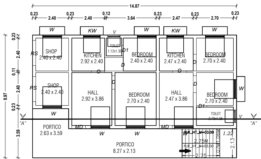
EX. GROUND FLOOR PLAN
