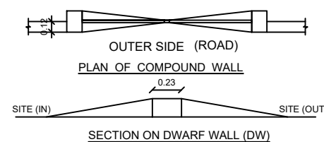
SECTION ON DWARF WALL (DW)
