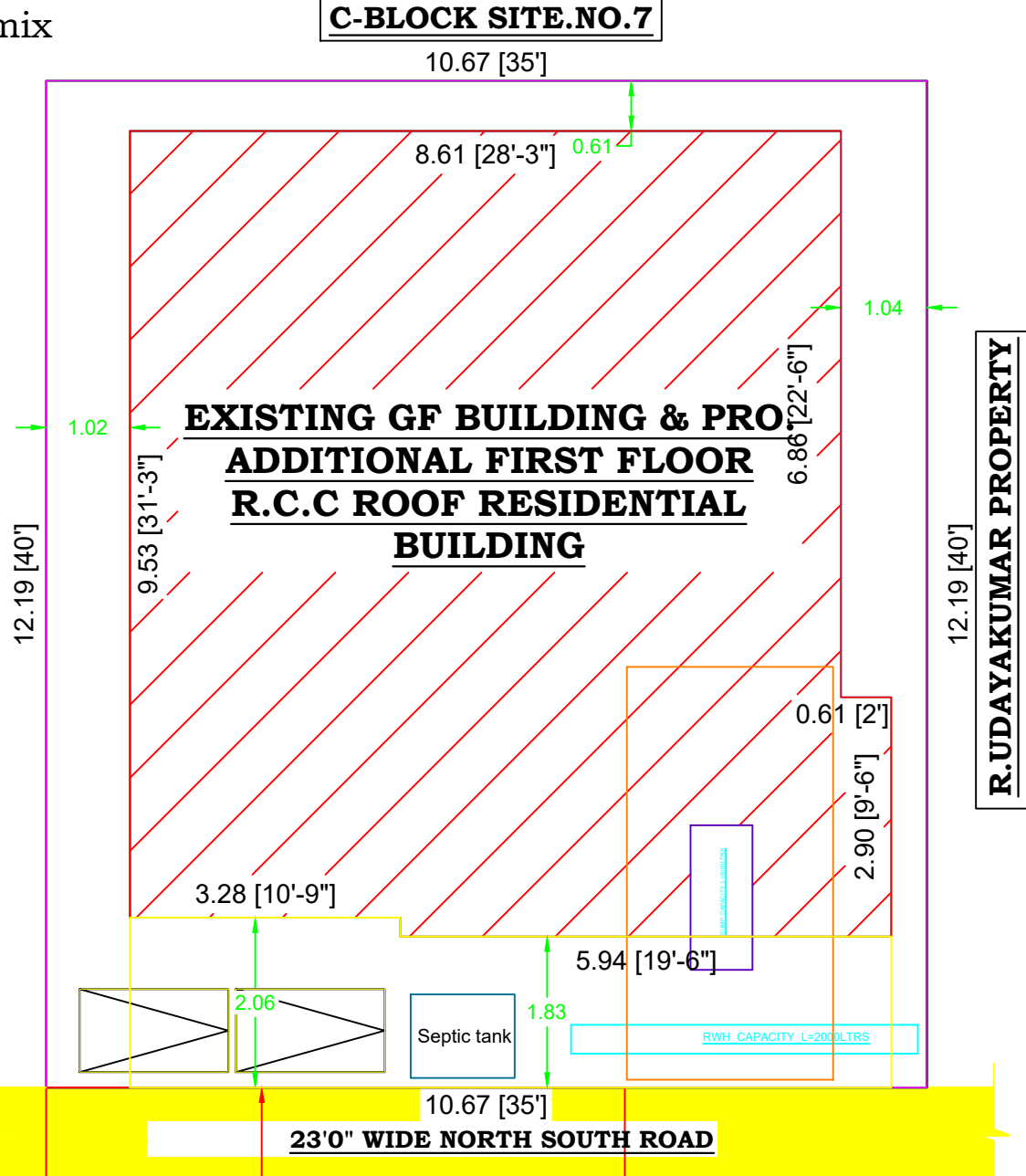
SITE PLAN
