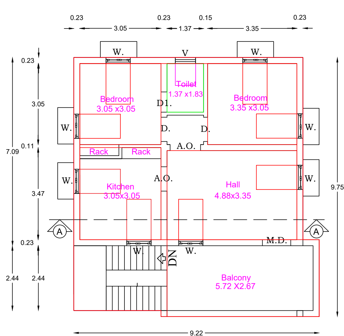
PROPOSED ADDITIONAL FIRST FLOOR PLAN
