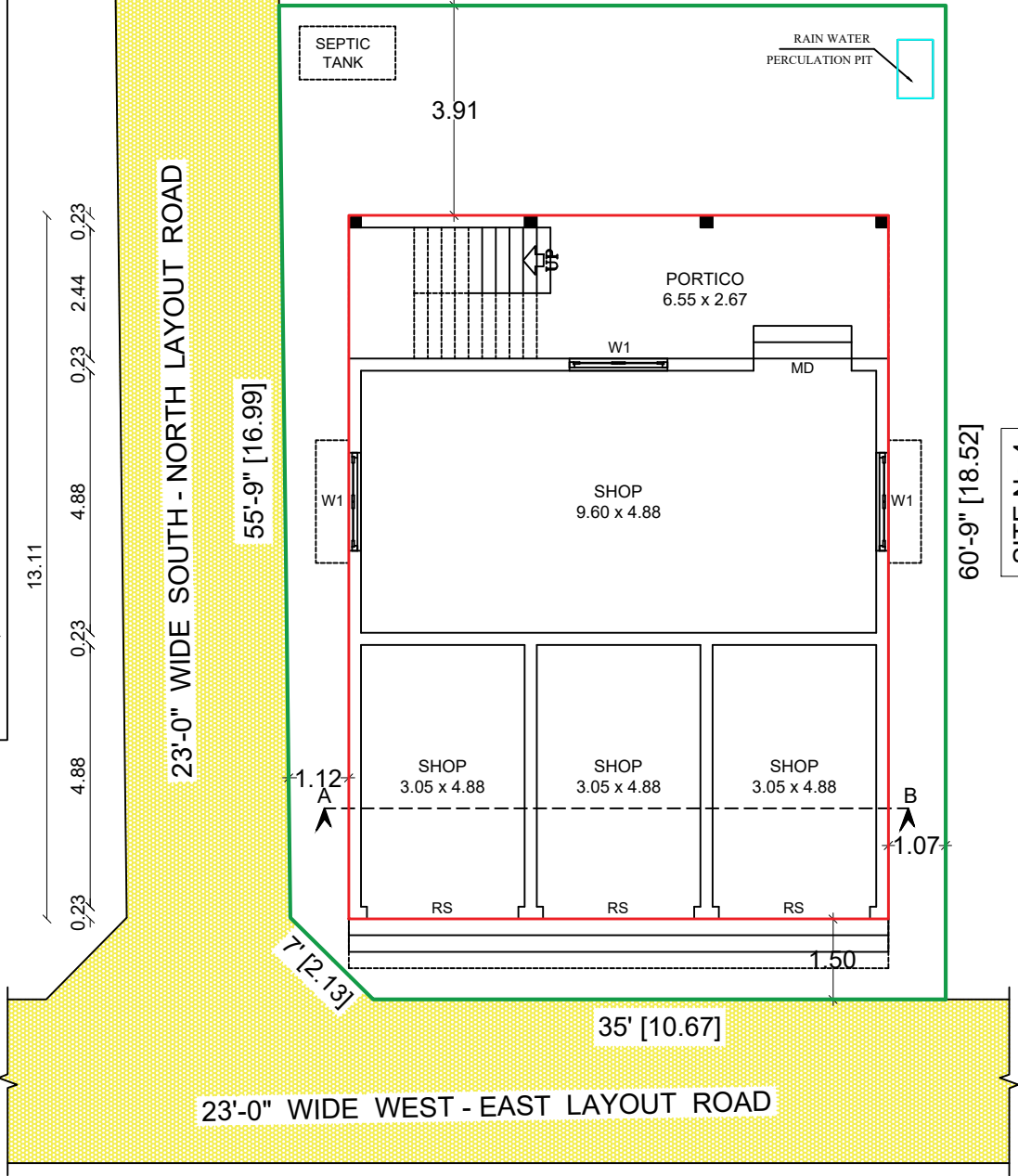
SITE CUM GROUND FLOOR PLAN
