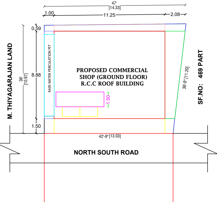
SITE PLAN
