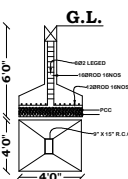
FOUNDATION DETAILS (NOT TO SCALE)
