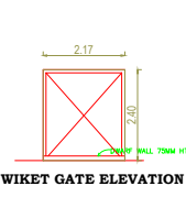
WICKET GATE ELEVATION
