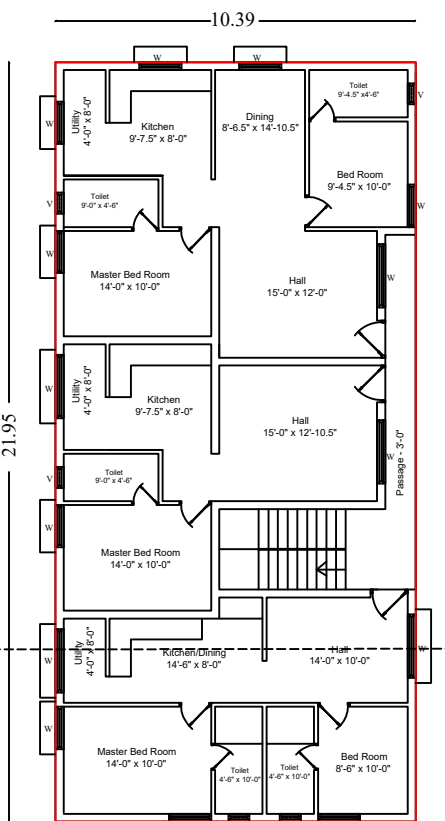
PRO. FIRST FLOOR
