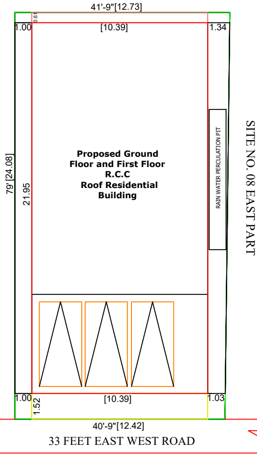
SITE PLAN
