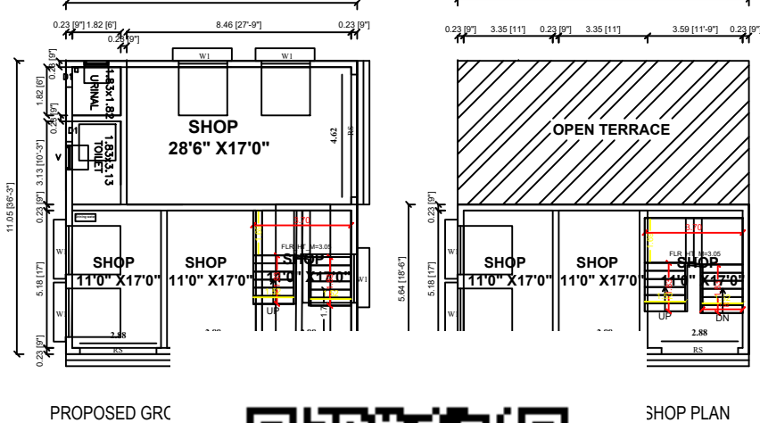
SHOP PLAN
