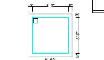
DETAILS OF COLLECTION SUMP FOR RAIN WATER HARVESTING OF ROOF TOP RAIN WATER RWH_CAPACITY_L=5000LTRS
