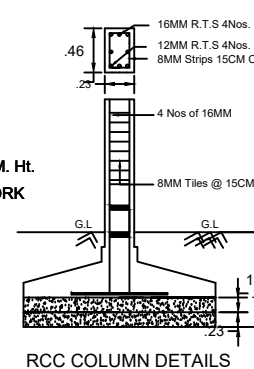
RCC COLUMN DETAILS
