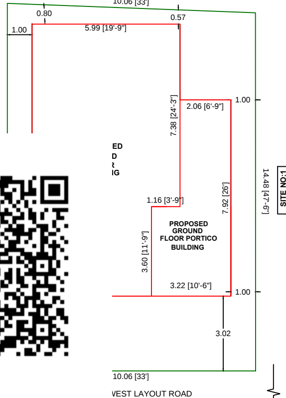
SITE PLAN
