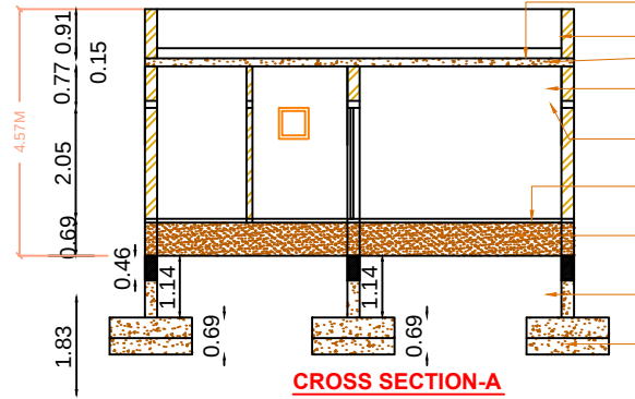
CROSS SECTION-A
