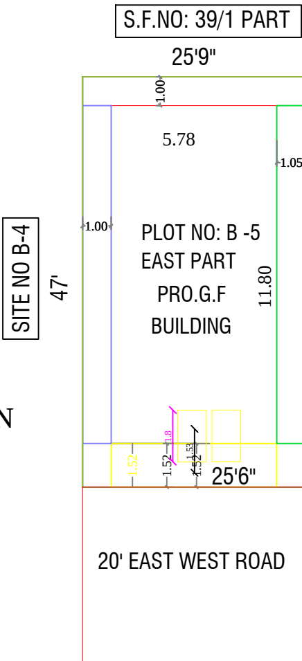
SITE PLAN
