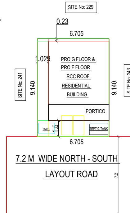
SITE PLAN
