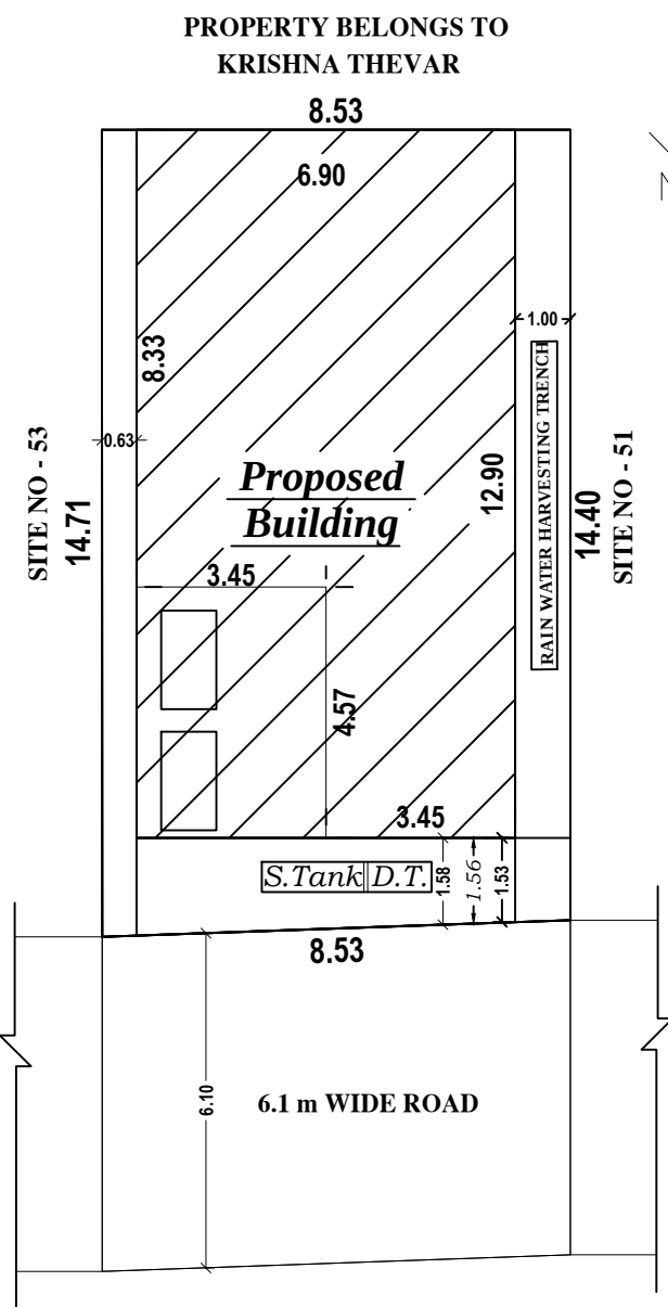
SITE PLAN
