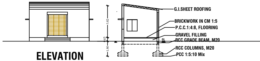
SECTION-AA'
