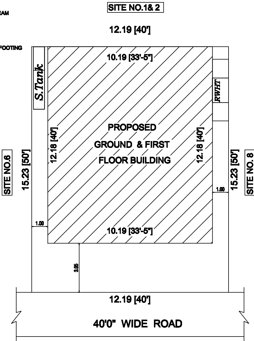
SITE PLAN
