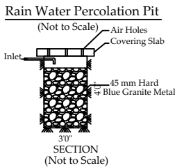
SECTION (Not to Scale)
