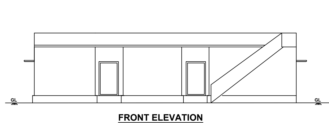
FRONT ELEVATION
