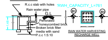
SECTION ON B1 B1
