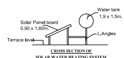
CROSS SECTION OF SOLAR WATER HEATING SYSTEM
