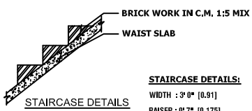
STAIRCASE DETAILS (NOT TO SCALE)
