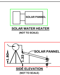
SOLAR WATER HEATER (NOT TO SCALE)
