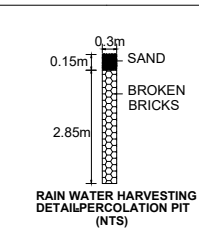
RAIN WATER HARVESTING DETAIL/PERCOLATION PIT (NTS)
