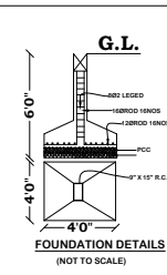
FOUNDATION DETAILS (NOT TO SCALE)
