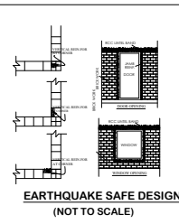
EARTHQUAKE SAFE DESIGN (NOT TO SCALE)
