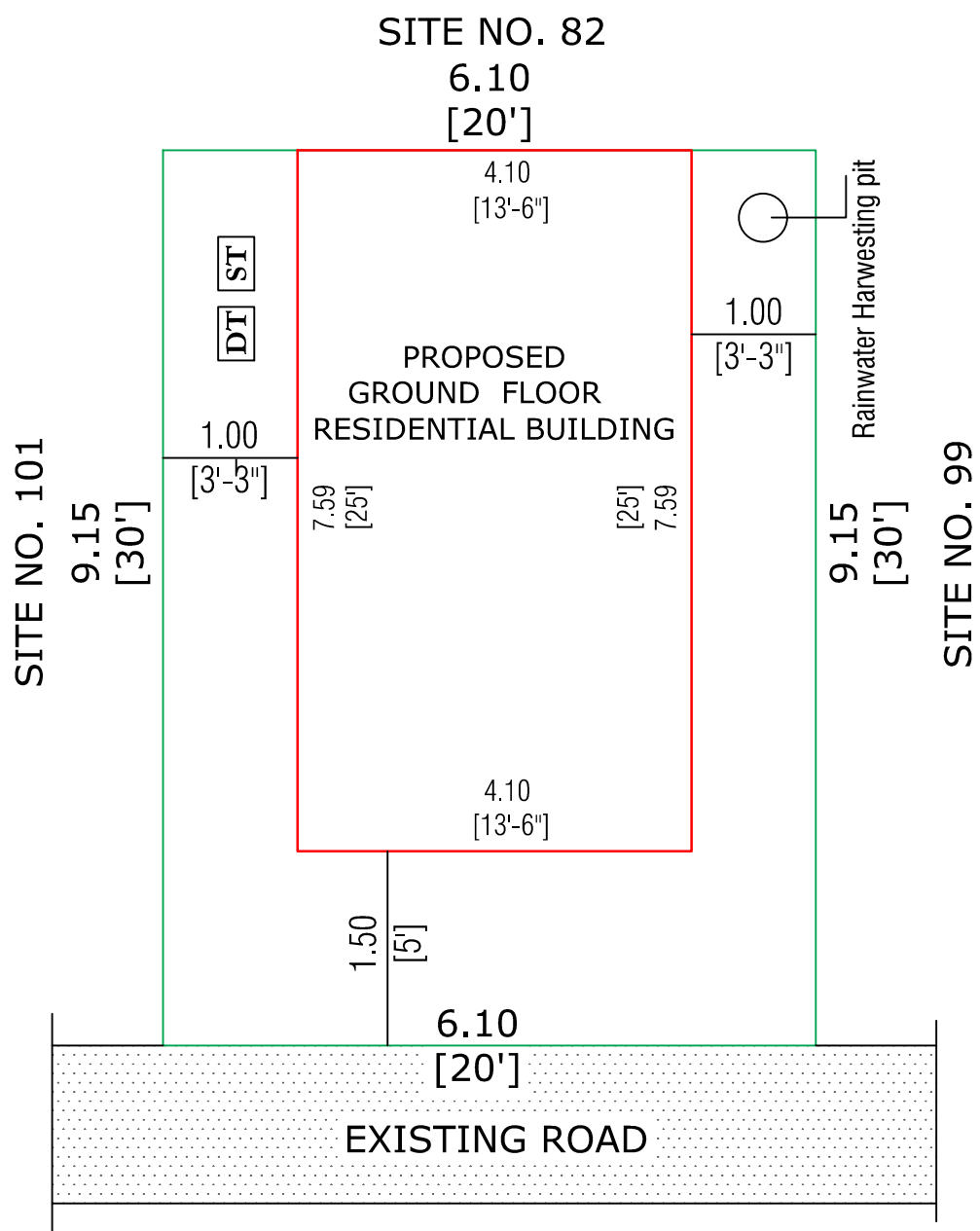
SITE PLAN (NOT TO SCALE)
